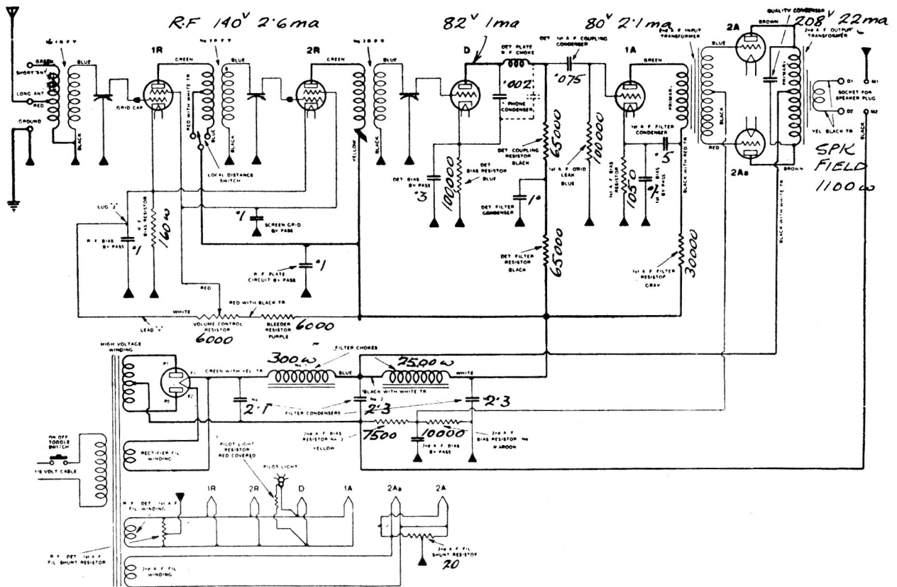
CIRCUIT DIAGRAM OF EARLY MODEL 55 AND 55-C WITH TRANSFORMER-COUPLED R. F. COILS. In some Model 55 and 55-C, a double "phone" condenser is used. In later Model 55 and 55-C the "phone" condenser is of the single type. For changes in the filament circuits, refer to Dealer Service Bulletin 6 of October 22, 1929.
