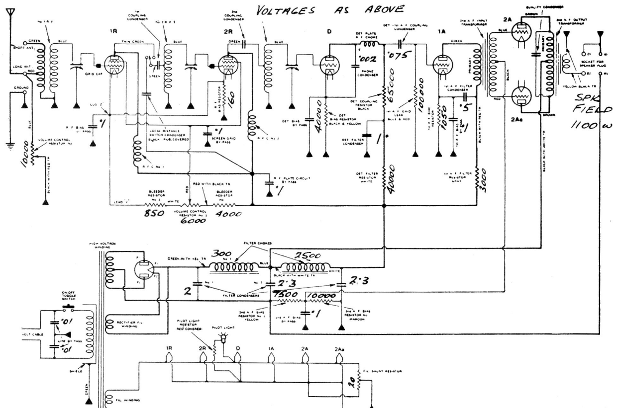
DIAGRAM OF LATER MODEL 55 AND 55-C WITH CAPACITY-COUPLED R. F. TRANSFORMERS. The changes shown above were made gradually, not all at one time
