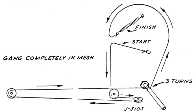
STRINGING DETAIL—MODEL RM-221AR
