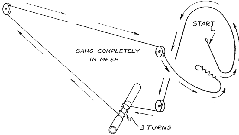
STRINGING DETAIL
