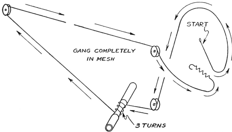
STRINGING DETAIL
