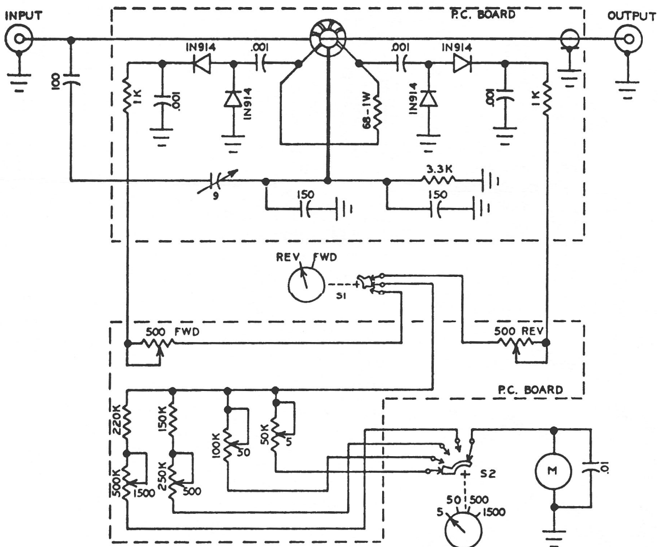
SCHEMATIC DIAGRAM - MODEL WM-1500 WATTMETER
