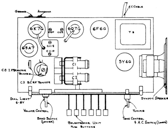
Top View of Model 5441
