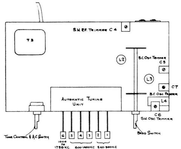
Bottom View of Model 5441
