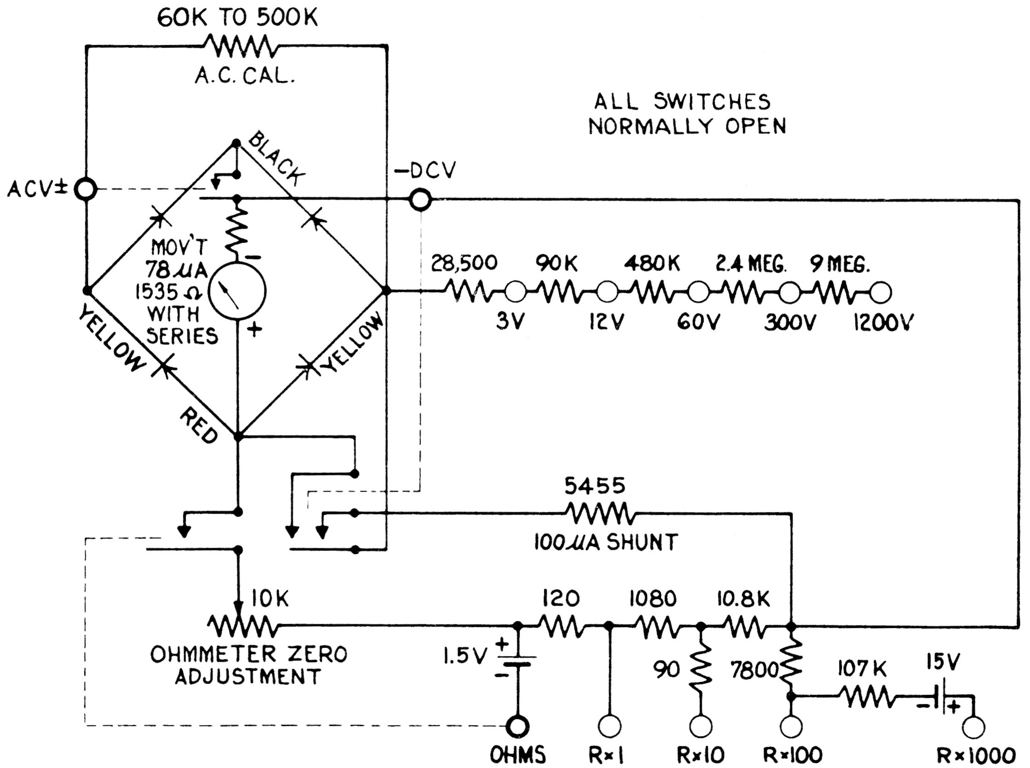
Figure 4. Overall Schematic Diagram, Model 355
