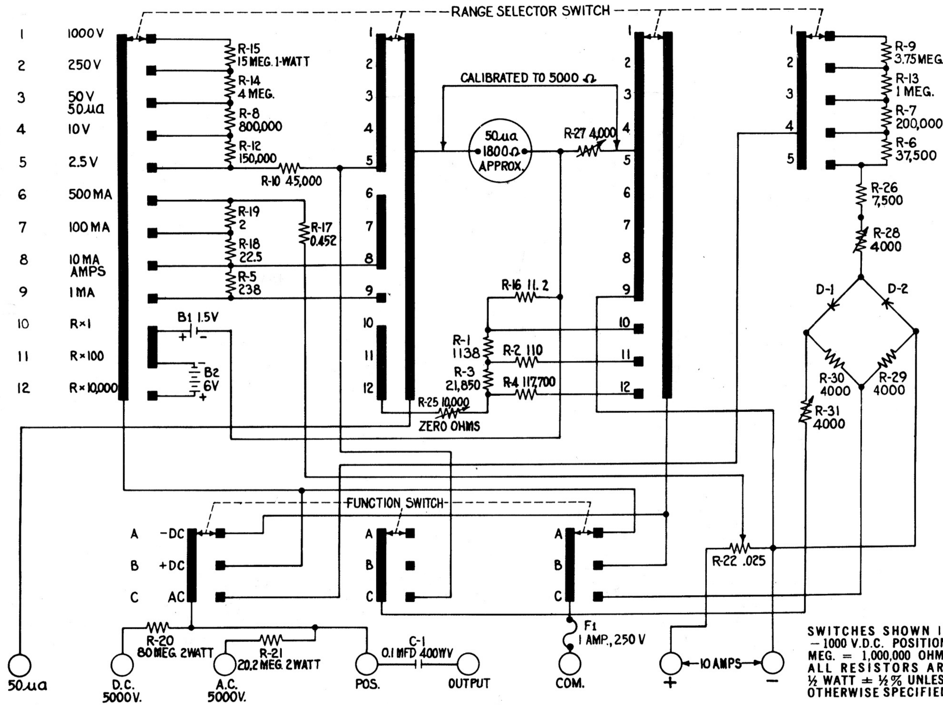
OVERALL SCHEMATIC, SIMPSON VOLT-OHM-MILLIAMMETER, MODEL 270
