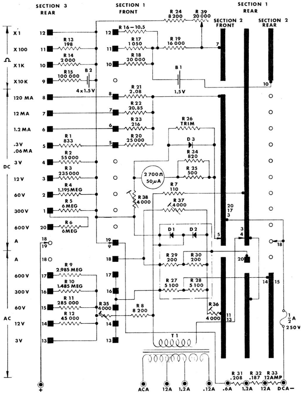
Figure 6-1. Schematic Diagram
