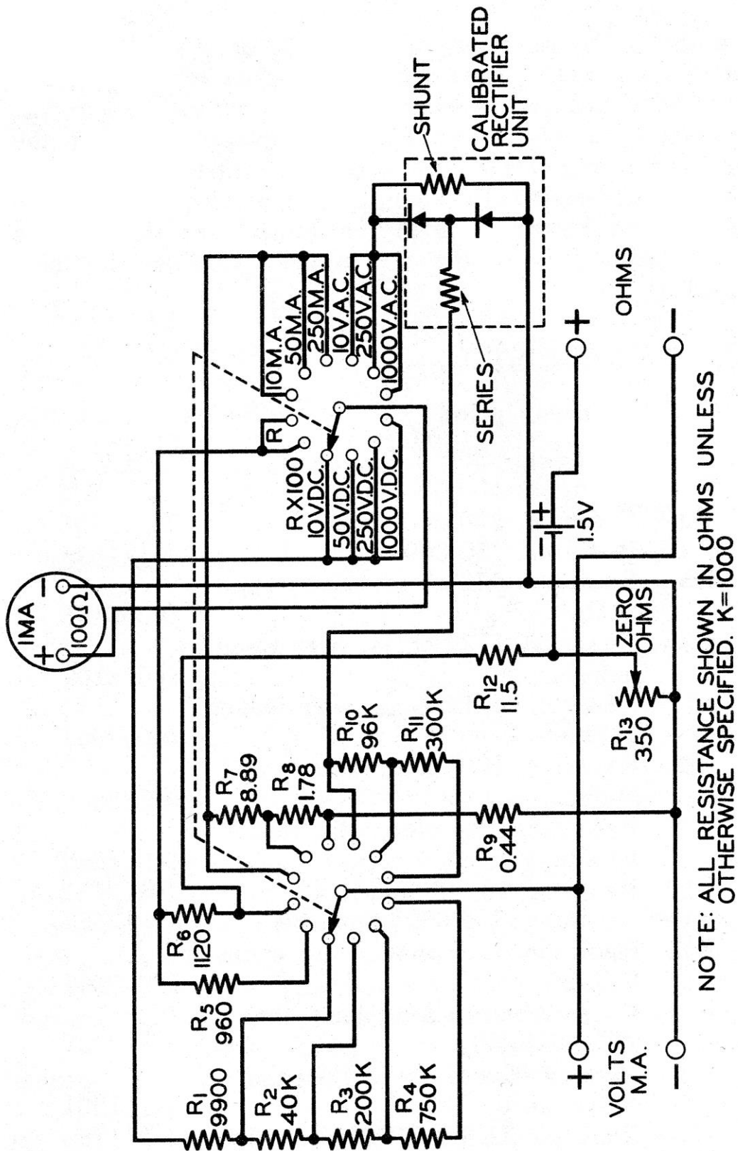
FIGURE 8. MODEL 230 VOLT-OHM-MILLIAMMETER, OVERALL SCHEMATIC DIAGRAM.
