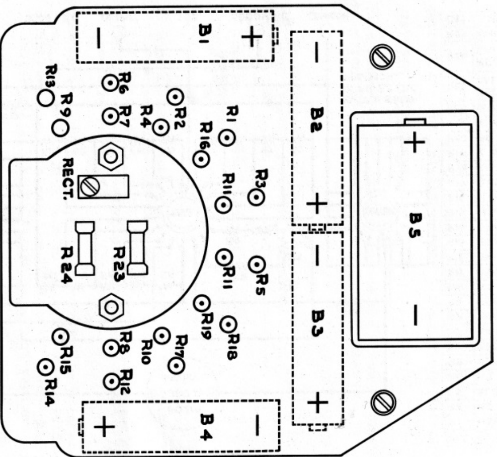
Figure 10a Model 221 Parts Layout--Rear View
