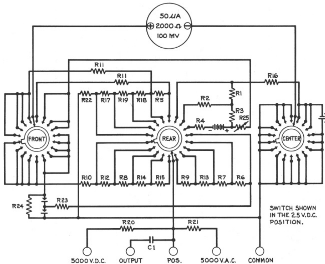
Figure 9 Model 221 Schematic Diagram
