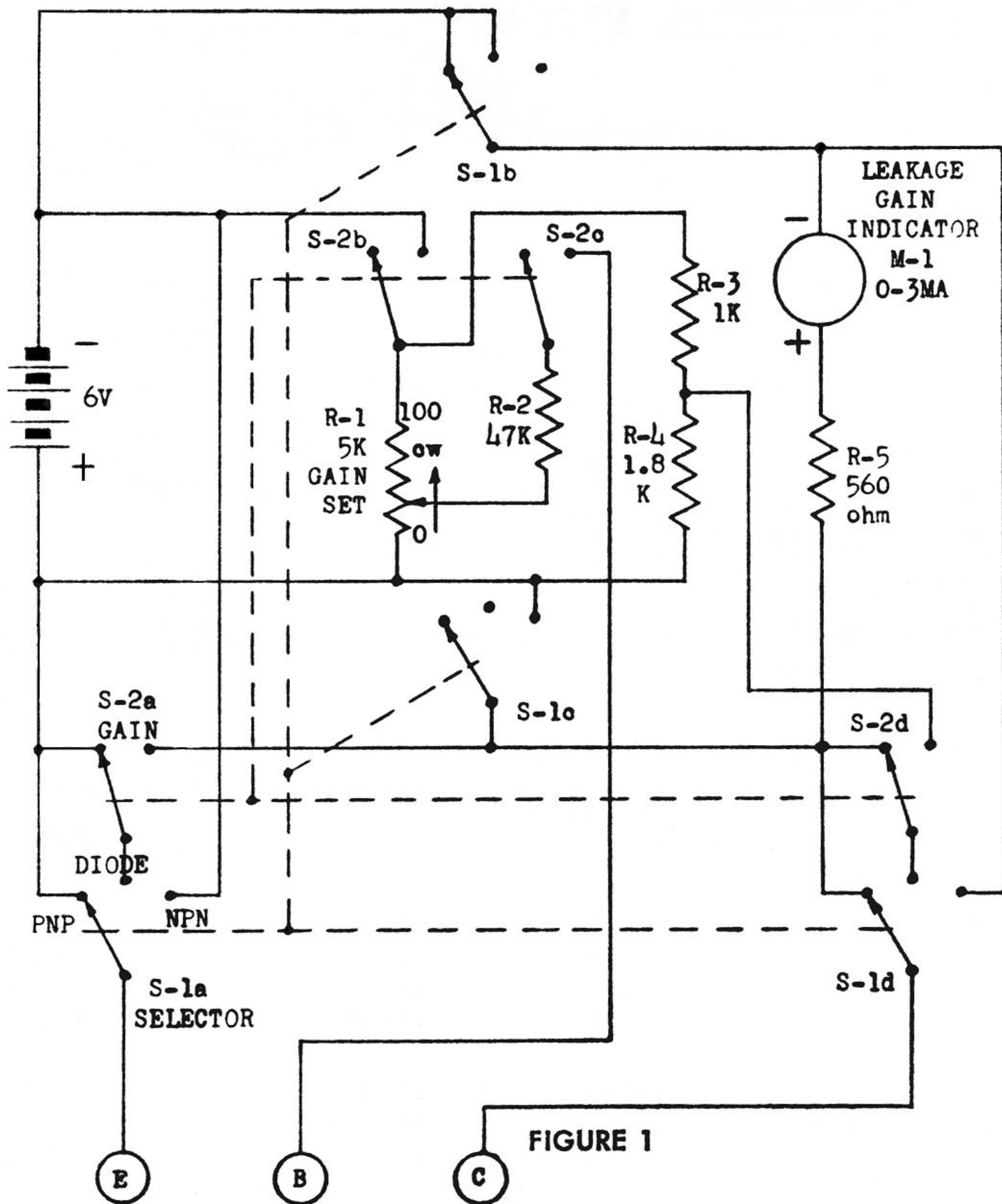
Sencore TDC22 Transistor Checker
