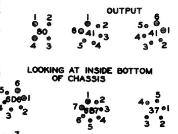
Terminal Layout for Voltage Measurement Chart.
