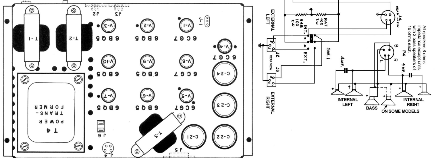
3 Channel Stereo Power Amplifier for RCA model SHC663
