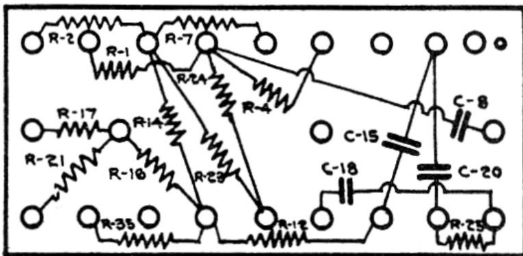
RESISTOR PANEL-MODEL 40
