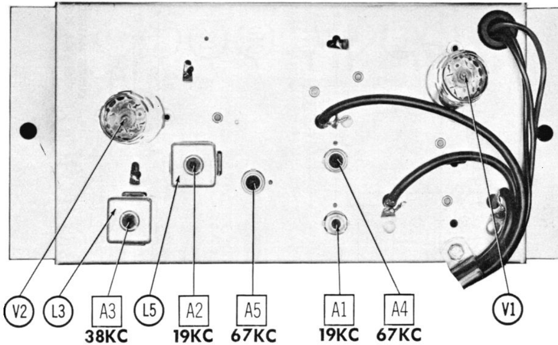
MULTIPLEX ALIGNMENT USING FM STEREO GENERATOR AND AUDIO OSCILLATOR
