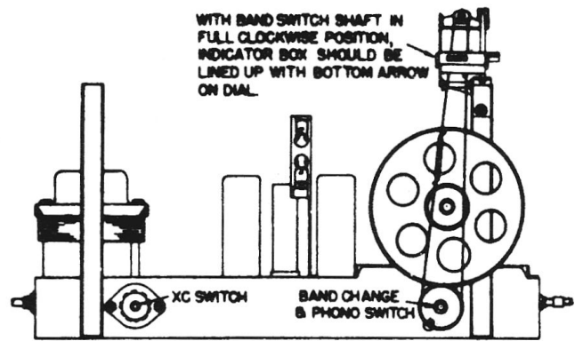
CM 25 CM 60 LAYOUT & DIAL CORD
