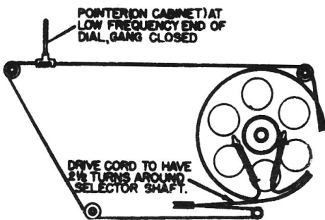
CM 70 LAYOUT & DIAL CORD
