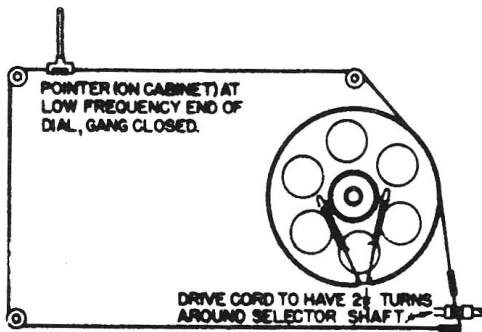
CM 25 CM 60 LAYOUT & DIAL CORD
