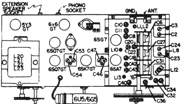
CM 70 LAYOUT & DIAL CORD
