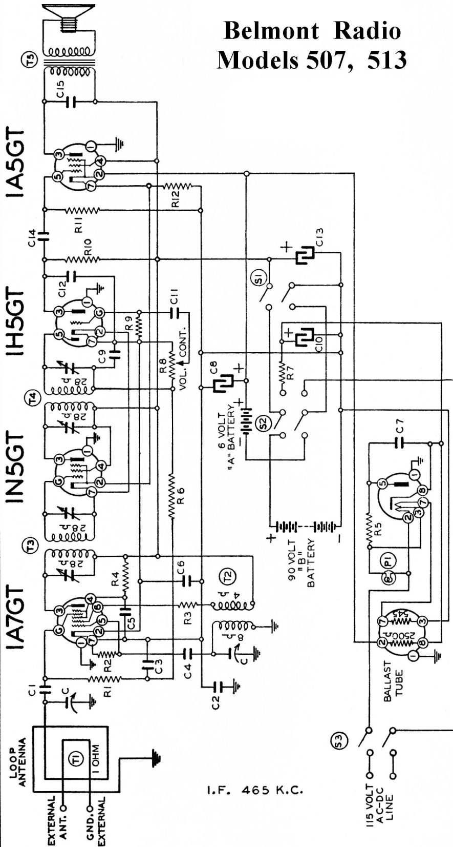
Circuit Diagram Ref. Part No. No.
