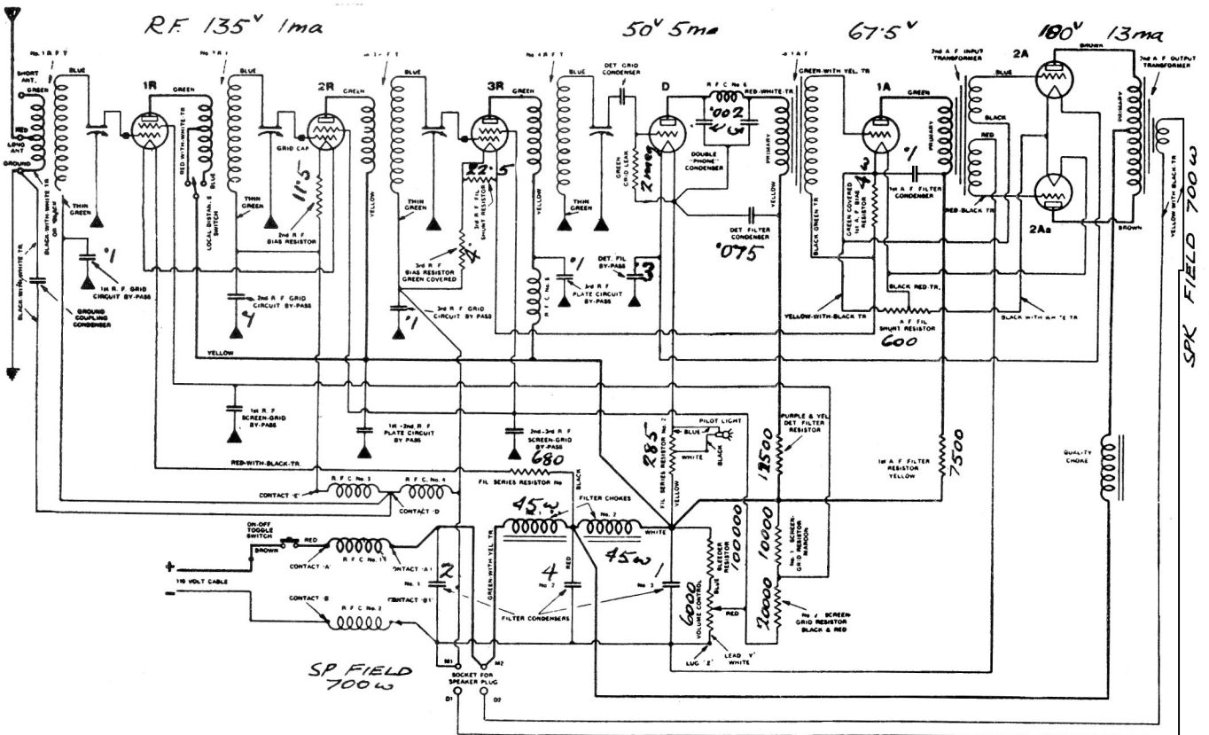
DIAGRAM OF EARLY MODEL 61 AND 61-C (DIRECT CURRENT).
