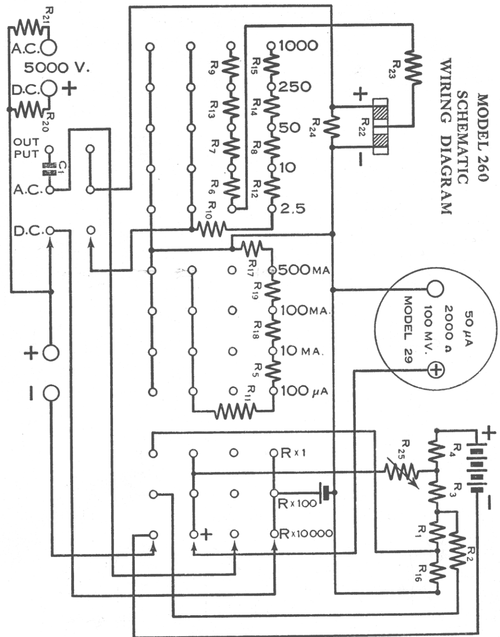
Figure 9 Model 260 Schematic Diagram
