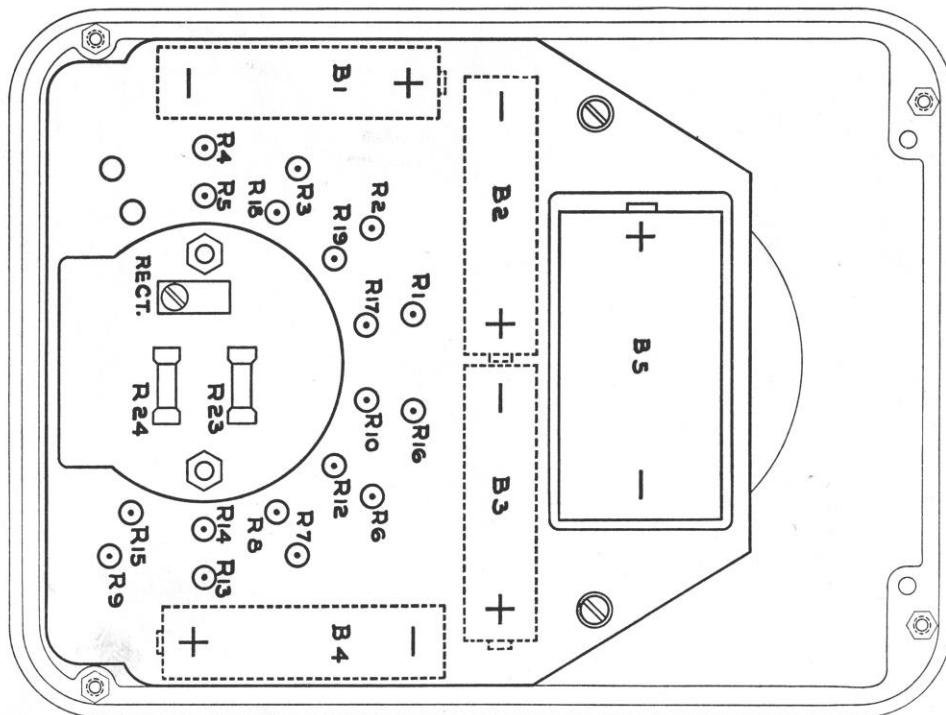
Figure 10a Model 215 Parts Layout—Rear View
