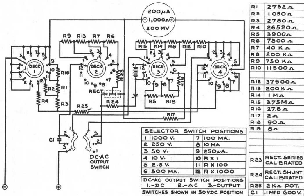
Figure 9 Model 215 Schematic Diagram
